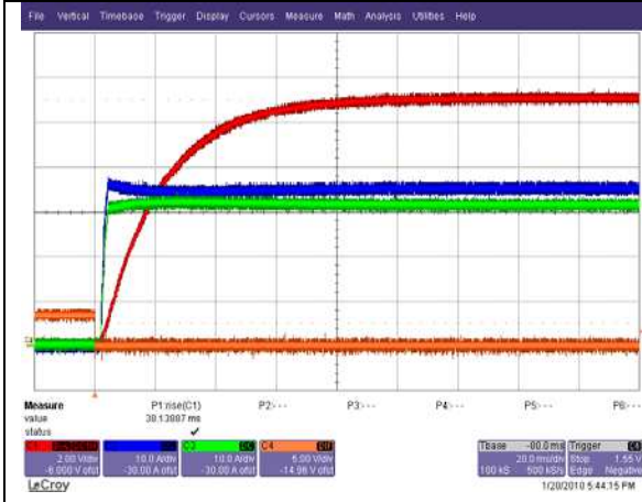
Start-up from on/off switch: 48Vin, Io=66A (200% Load) Ch. 1: Vo Ch. 2: Io1 Ch. 3: Io2 Ch. 4: ON/OFF
