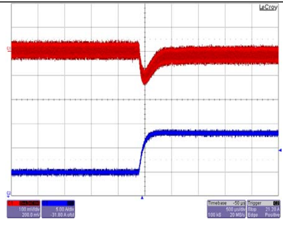
Load Transient Response with Droop Disabled. Load Step: 50% to 75% Ch. 1: Vo Ch. 2: Io
