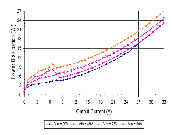
Power Dissipation vs. Vin (test in socket, no base-plate)
