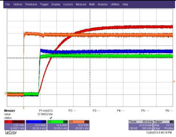
Start-up from Vin: 48Vin, Io=66A (200% Load) Ch. 1: Vo Ch. 2: Io1 Ch. 3: Io2 Ch. 4: Vin
