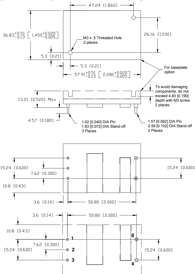
Recommended hole pattern (top view)
