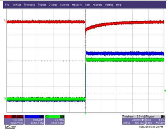
Load Transient Response. Load Step: 0A to 66A, 0.1A/us slew rate. Ch. 1: Vo Ch. 2: Io1 Ch. 3: Io2
