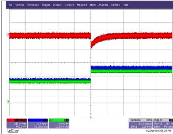
Load Transient Response. Load Step: 33A to 49.5A, 0.1A/us slew rate. Ch. 1: Vo Ch. 2: Io1 Ch. 3: Io2
