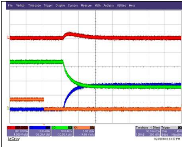
Start-up with back-biasing: Vin=48V, Io=33A Ch. 1: Vo Ch. 2: Io1 Ch. 3: Io2 Ch. 4: ON/OFF
