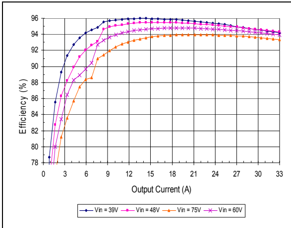
Typical Efficiency vs. Vin (test in socket, no base-plate, Vo measured at socket terminals)
