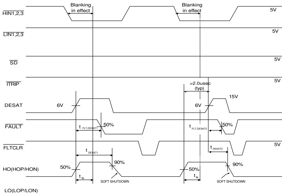
Figure 5. DESAT Timing
