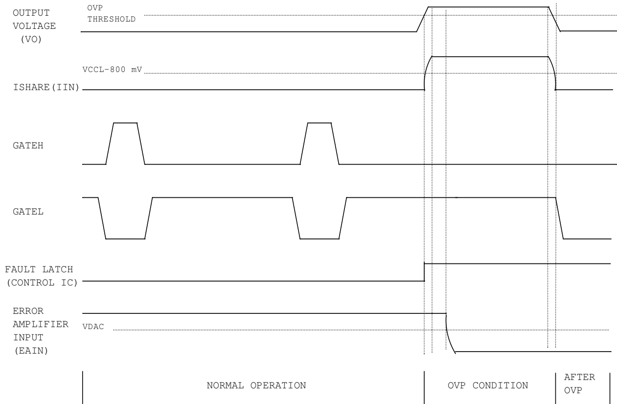
Figure 7 - Over-voltage protection waveforms
