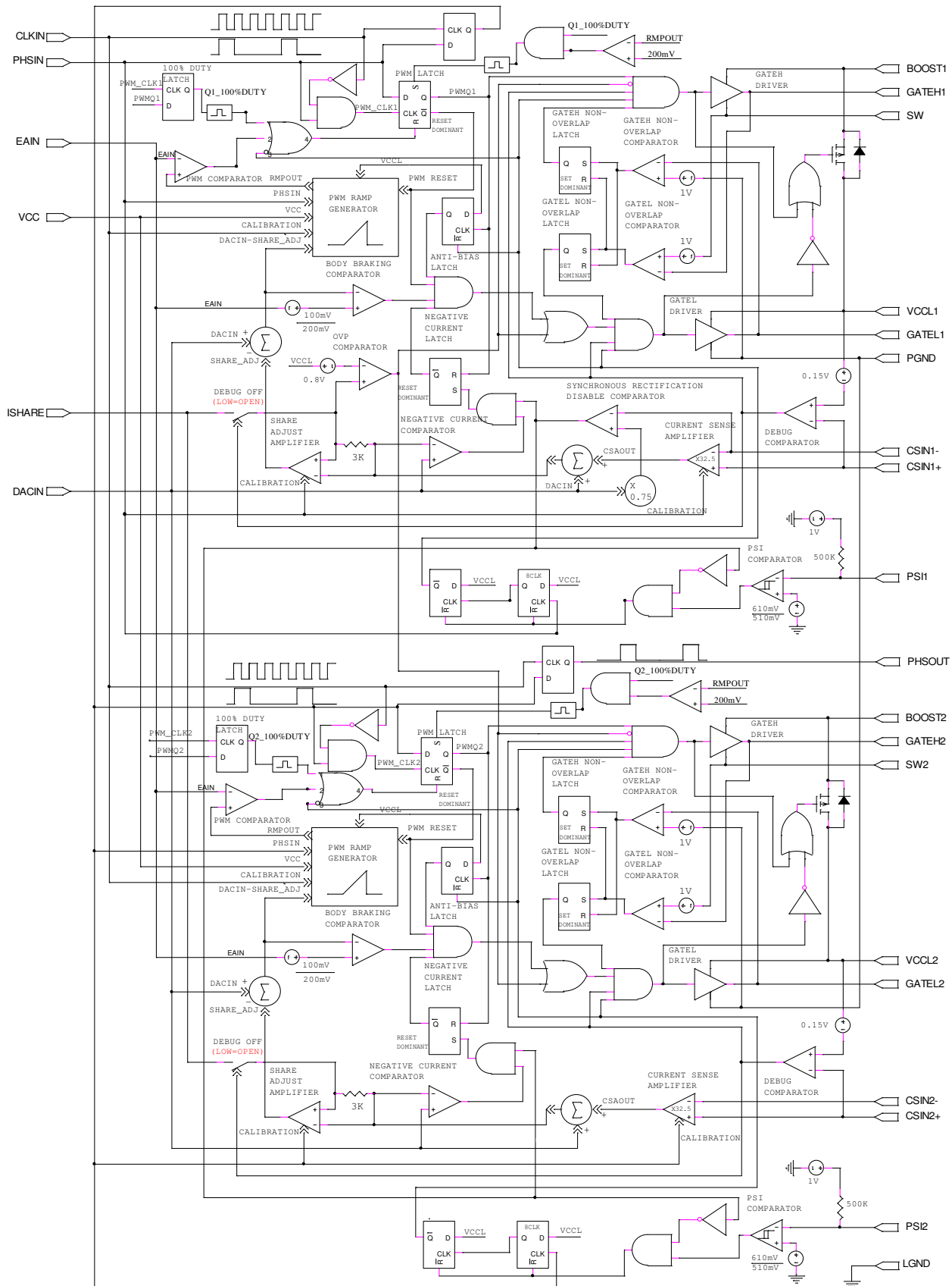
Figure 6 – IR3527 Block diagram
