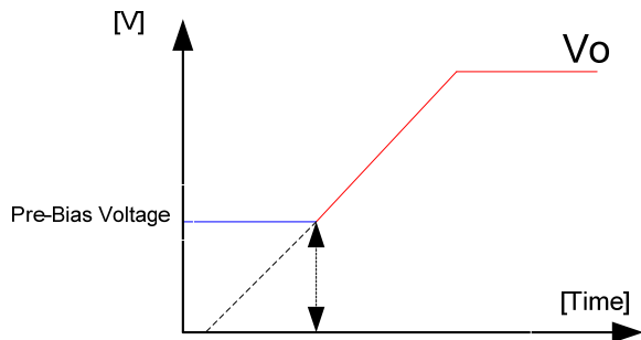
Fig. 4. Pre-Bias startup
