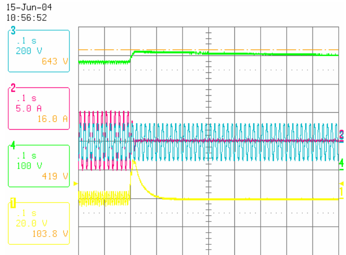
300W to No Load Step @ 90VAC
