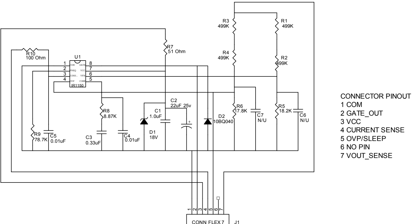
Figure 1 – IRAC1150-D2 Control Board Schematic Diagram
