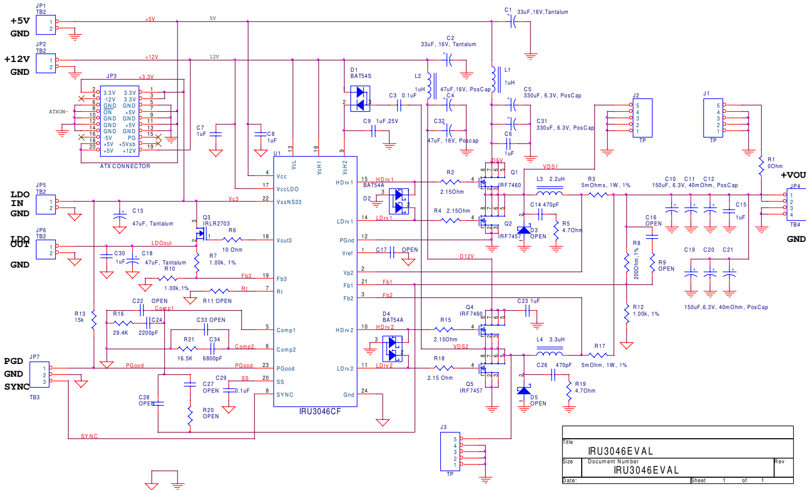
Figure 3 - Schematic of evaluation-board for IRU3046.
