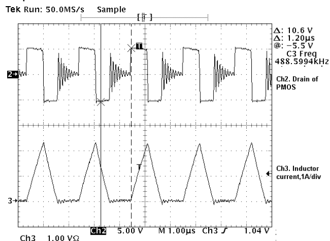
Operation waveforms with 250mA load (normal operation)
