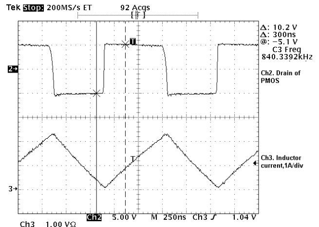
Operation waveform with 450mA, the boundary of continuous mode and discontinuous mode. The output start out of regulation
