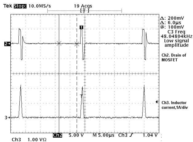
Operation waveform at 20mA load.
