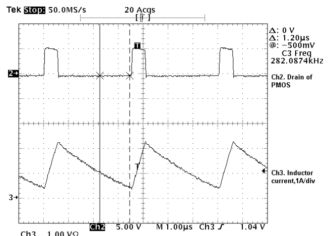
Operation waveform with short output.
