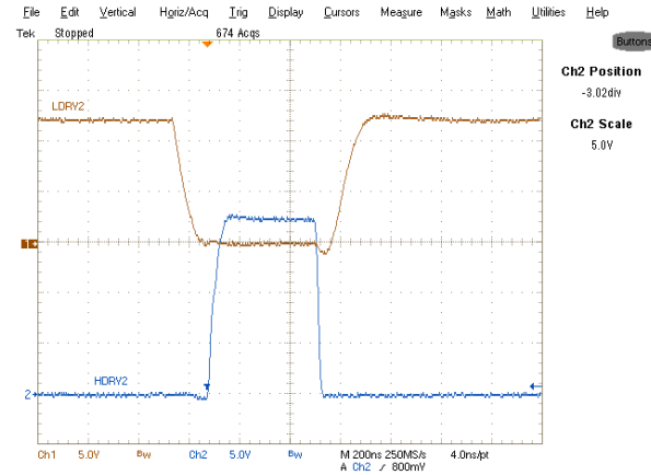
Fig. 28: HDRV2 and LDRV2 at 20A. Ch 1 : LDRV2, Ch 2 : HDRV2
