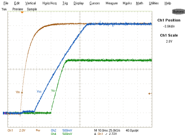
Fig.13: Start-up sequence at no load. Ch 1 : V_{in} , Ch 2 : V_{ss} , Ch 4 : V_o
