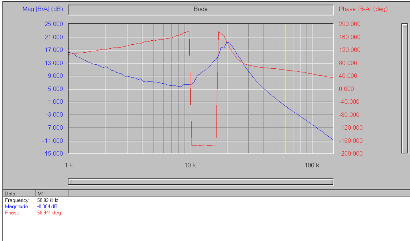
Fig.16: Bode Plot at 8A load (sourcing current) shows a bandwidth of 59kHz and phase margin of 59 degrees
