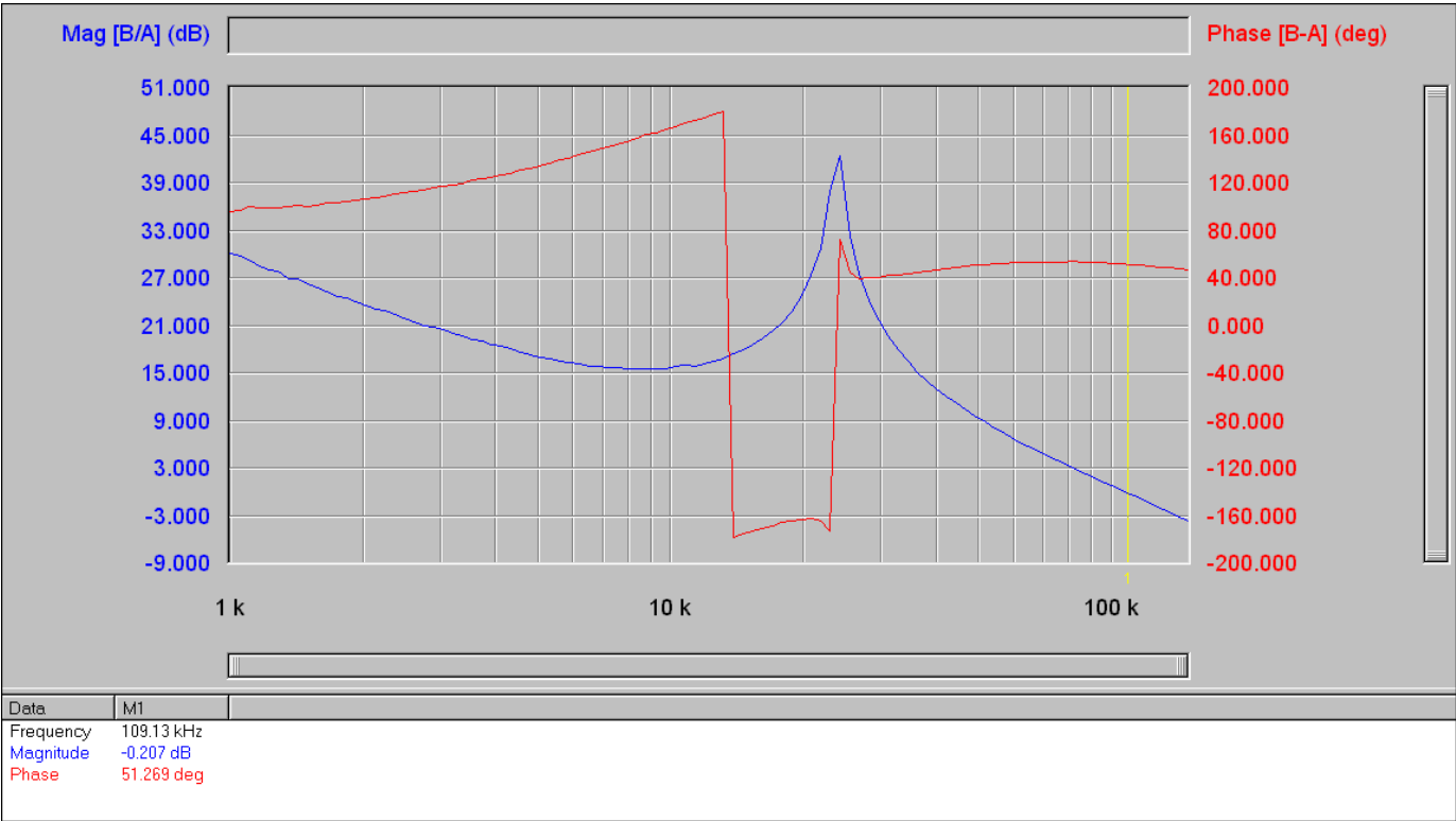
Fig. 14: Bode Plot at 12A load shows a bandwidth of 109kHz and phase margin of 51 degrees
