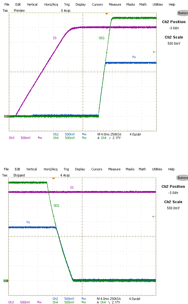
Fig. 18: Simultaneous Tracking a 3.3V input at power-up and shut-down Ch2: SS (1.8V) Ch3:Vo Ch4: SEQ
