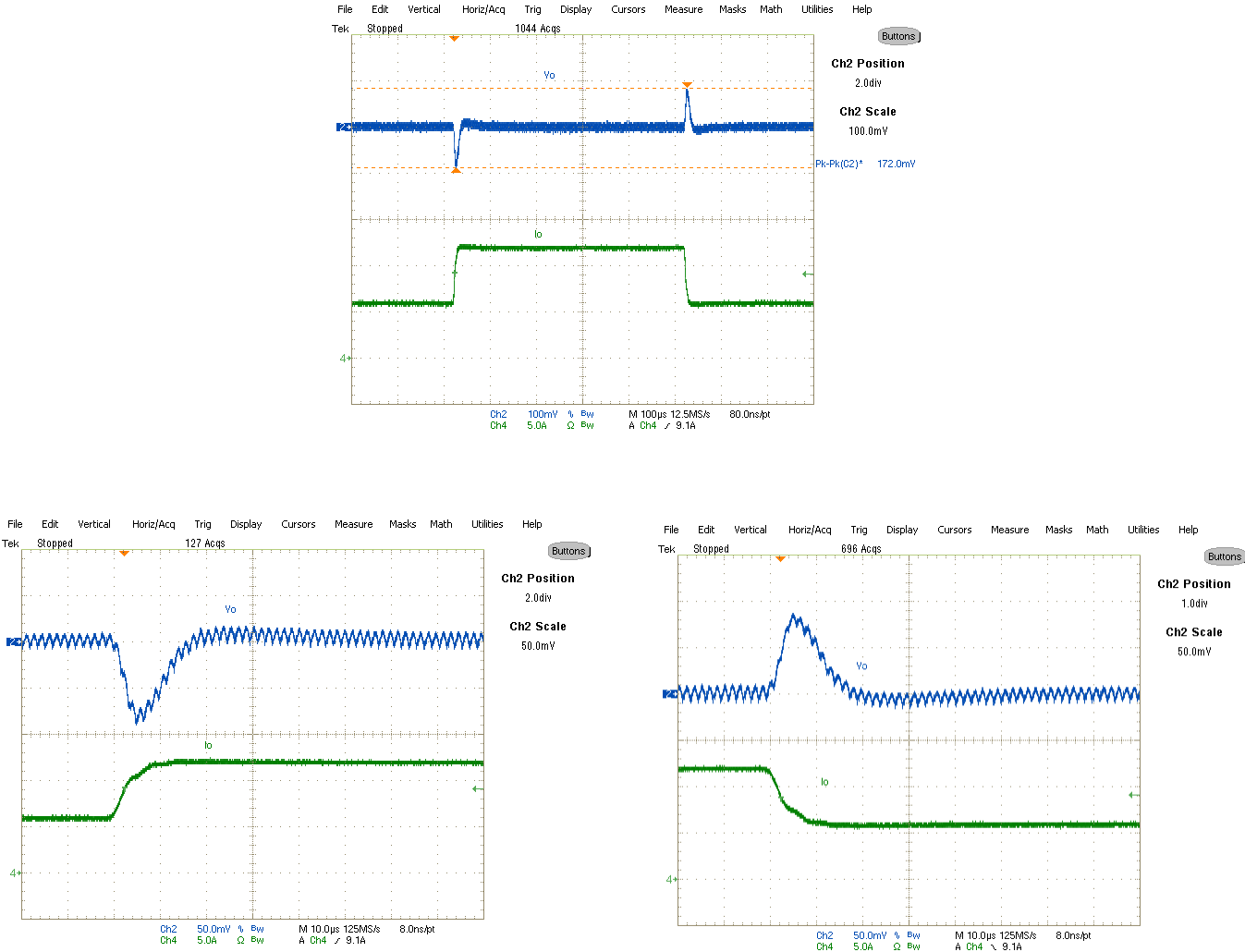
Fig. 13: Transient Response, 6A to 12A step 2.5A/μs Ch 2 :V out , Ch 4 :I out
