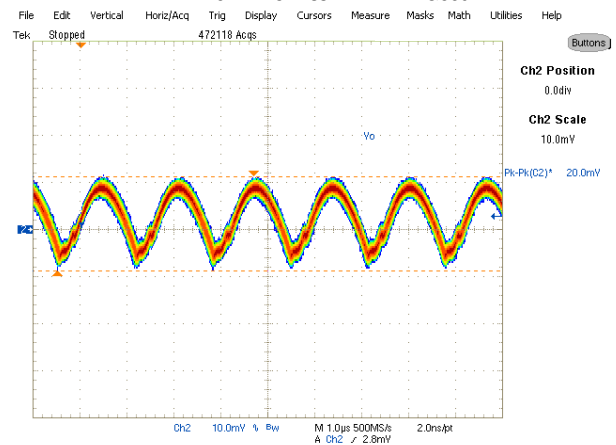
Fig. 10: Output Voltage Ripple, 12A load Ch 2 : V_{out}
