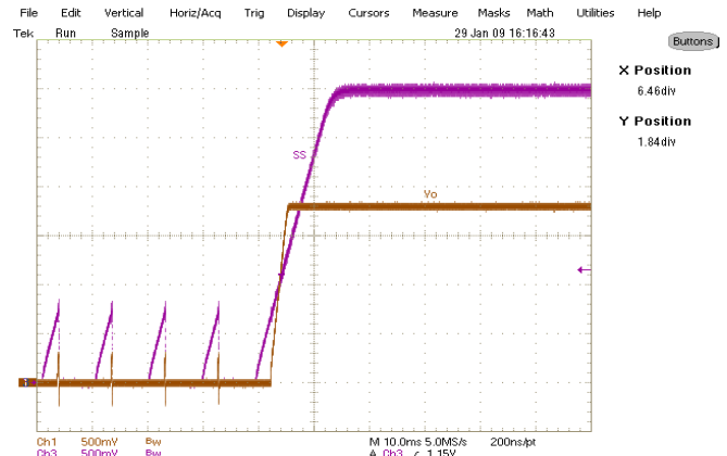
Fig. 22. Short (Hiccup) Recovery Ch 1 :V o , Ch 3 :V ss
