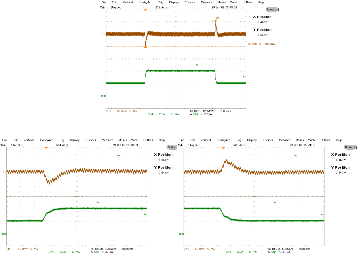
Fig. 23. Transient Response, 2A to 4A step 2.5A/\mu s Ch_1:V_o , Ch_4:I_o
