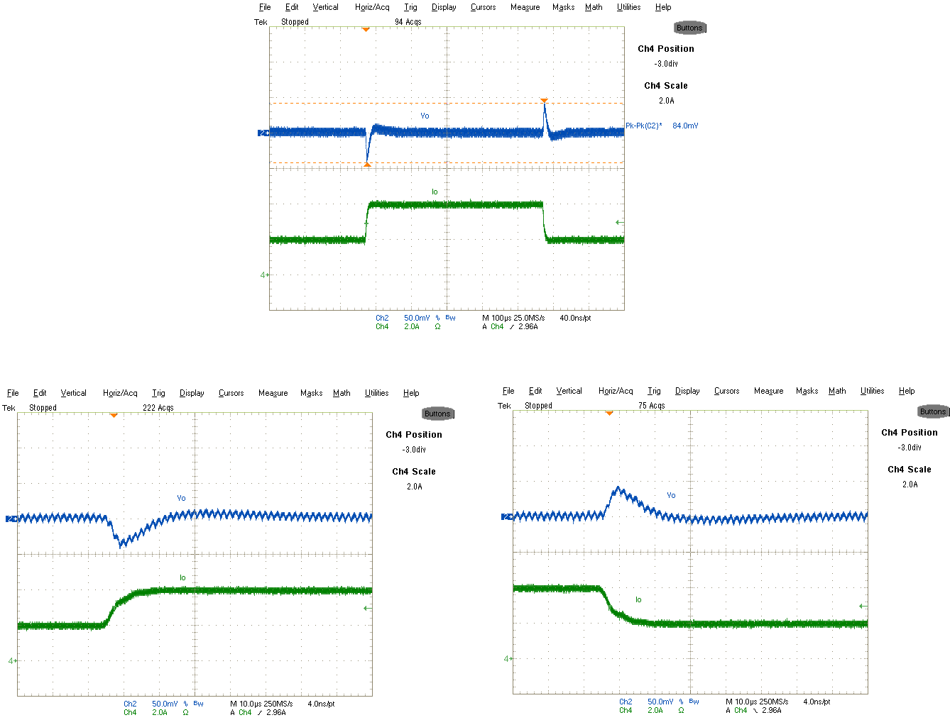
Fig. 23. Transient Response, 2A to 4A step 2.5A/μs Ch 2 :V o , Ch 4 :I o
