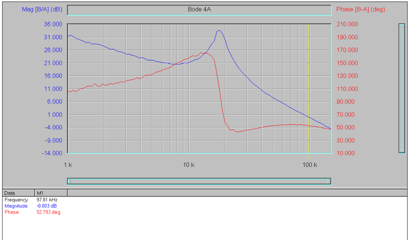
Fig. 24. Bode Plot at 4A load shows a bandwidth of 98kHz and phase margin of 53 degrees
