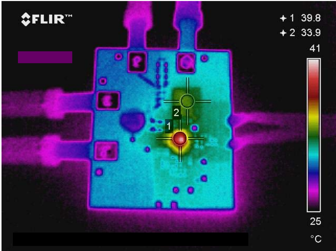
Fig. 17: Thermal Image at 4A load Test points 1 and 2 are IR3842W and inductor, respectively.
