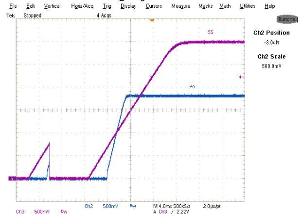
Fig. 22. Short (Hiccup) Recovery Ch 2 :V o , Ch 3 :V ss
