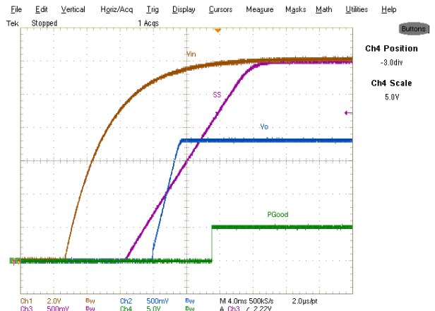
Fig. 18. Start up at 4A Load, Ch 1 :V in , Ch 2 :V o , Ch 3 :V ss , Ch 4 :V PGGood
