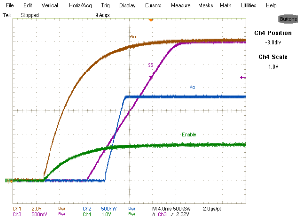
Fig. 17. Start up at 4A Load Ch 1 :V in , Ch 2 :V o , Ch 3 :V ss , Ch 4 :Enable
