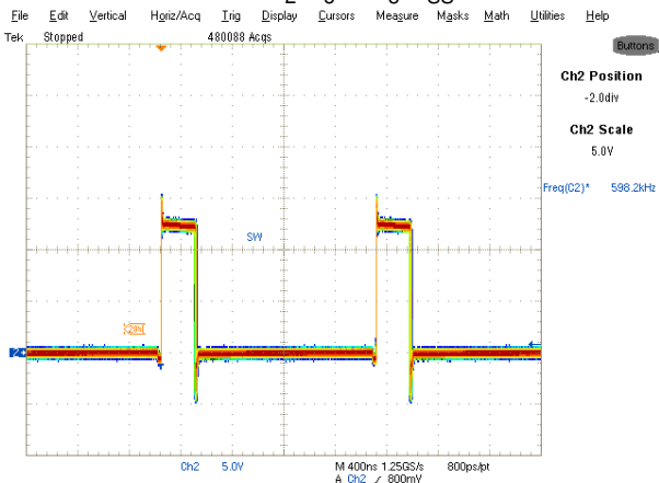
Fig. 21. Inductor node at 4A load Ch 2 :LX
