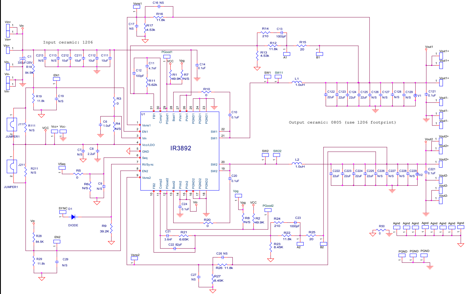
Fig.6: Schematic of the IRDC3892 evaluation board
