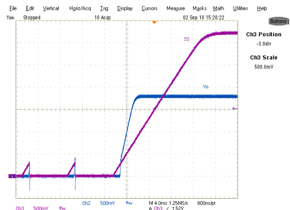
Fig. 7: Short (Hiccup) Recovery Ch 2 :V out , Ch 3 :V ss
