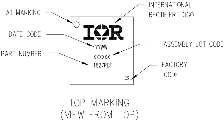
Fig. 19. Part Marking
