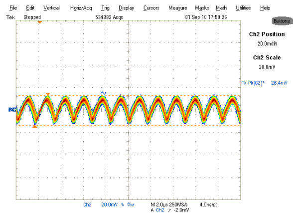
Fig. 5: Output Voltage Ripple, 25A load Ch 2 : V out
