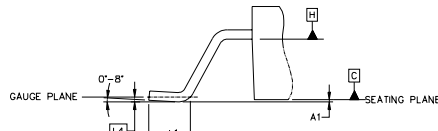
DETAIL "A" ROTATED 90° SCALE 8:1
