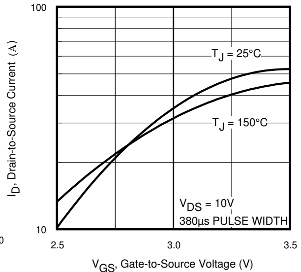
Fig 8. Typical Transfer Characteristics
