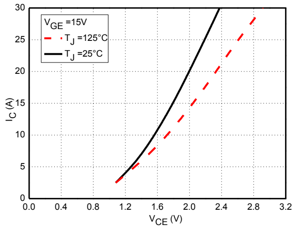
Fig.1 Typical IGBT Saturation Characteristics
