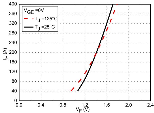
Fig.3 Typical Diode Forward Characteristics
