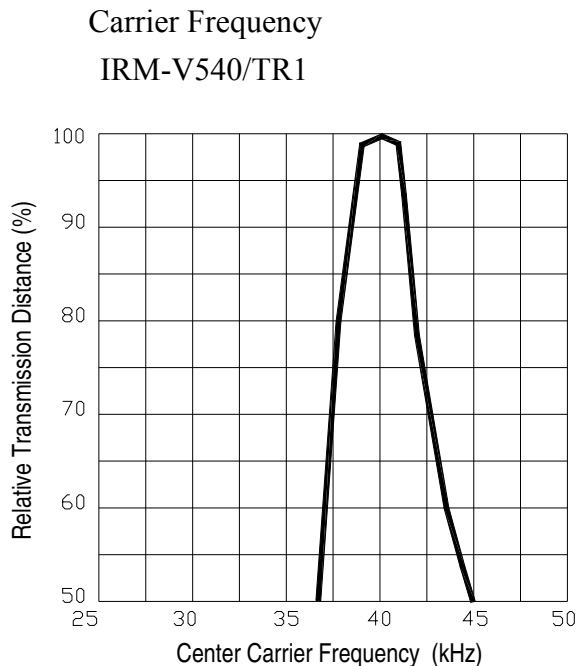
Fig.-9 Relative Transmission Distance vs. Center Carrier Frequency Fig.-9 Relative Transmission Distance vs. Center
