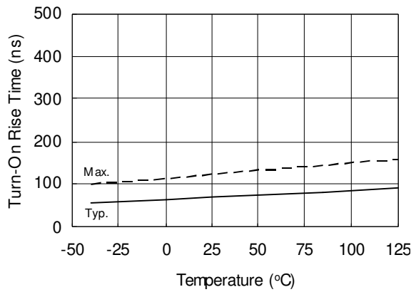
Figure 19A. Turn-On Rise Time vs. Temperature
