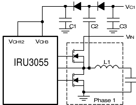
Figure 11 - Supply V CH12 , V CH3 with charge pump configuration.
