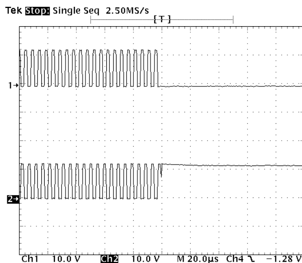
Figure 19 - Gate signals when SS pin pulls low.
