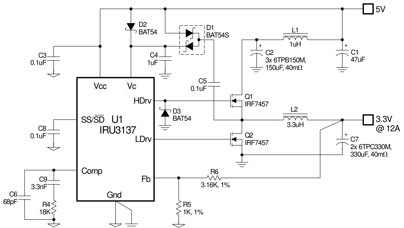
Figure 11 - Typical application of IRU3137 in an on-board DC-DC converter using a single 5V supply.
