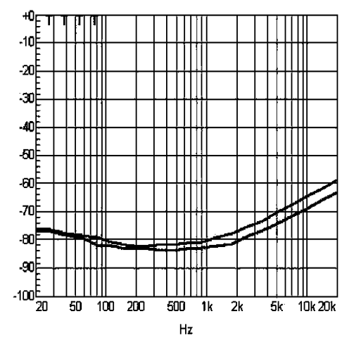
Figure 19 PSRR vs. Freq SE mode, 3V, 320Ohm, 200mVpp Input terminated
