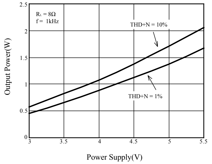
Figure 11 Output Power vs. Power Supply
