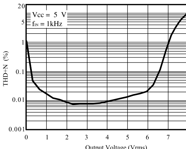
Figure 7 THD+N vs. Output Voltage( R_L = 1\mu F + 10\Omega )
