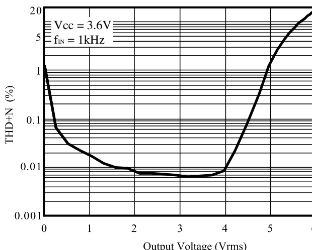
Figure 5 THD+N vs. Output Voltage( R_L = 1\mu F + 10\Omega )
