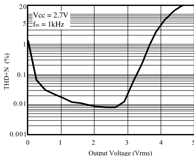
Figure 3 THD+N vs. Output Voltage( R_L = 1\mu F + 10\Omega )
