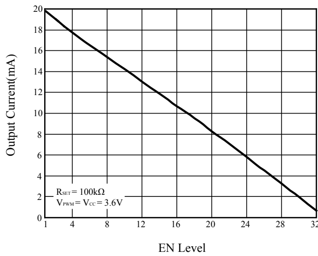
Figure 4 EN pin dimming
