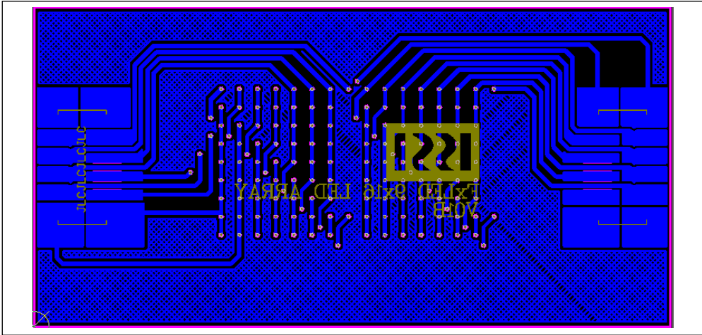
Figure 11: LED Board PCB Layout - Bottom Layer
