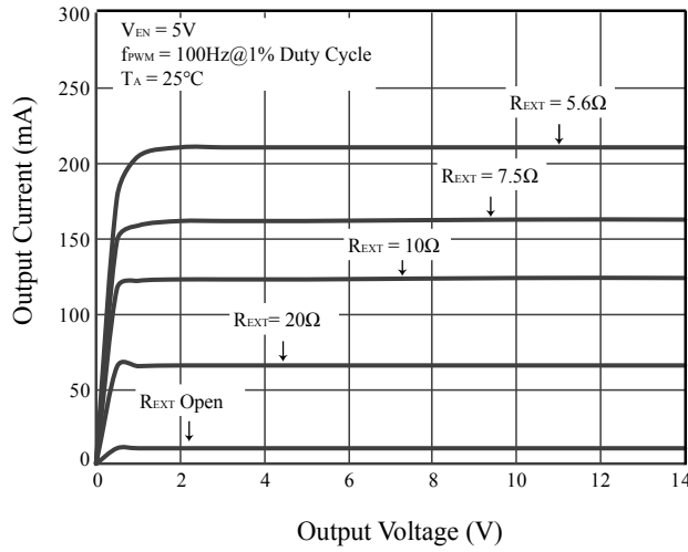
Figure 23 I_{OUT} vs. V_{OUT}
