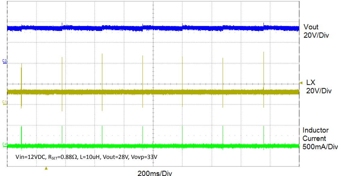
Figure 13 OVP waveform
