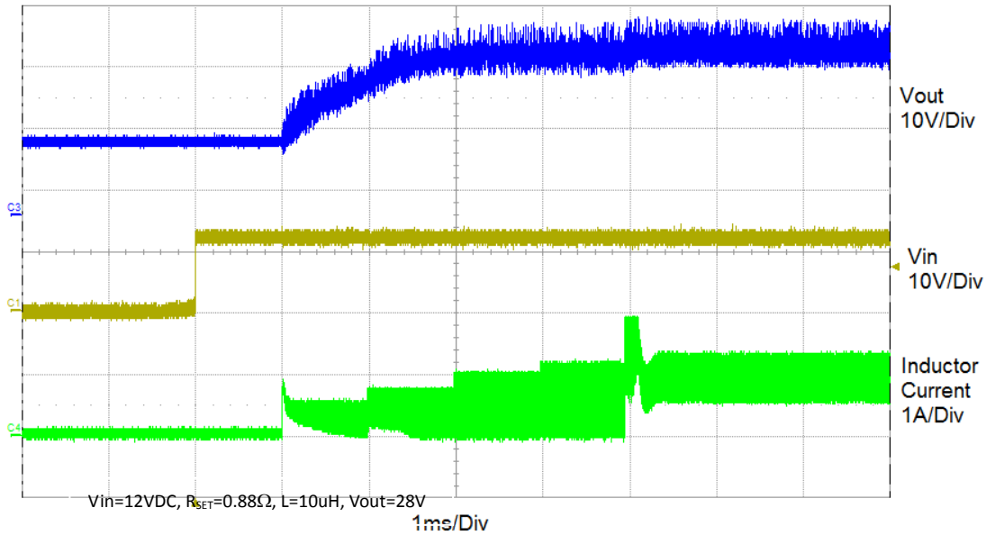
Figure 11 Soft-start waveform
