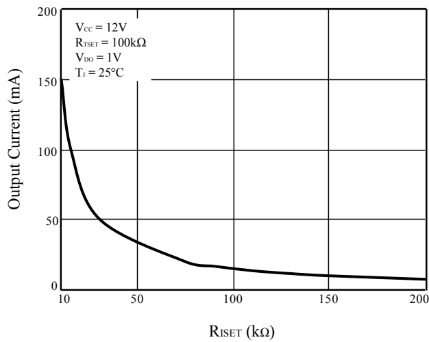
Figure 4 Output Current vs. R_{ISET}
