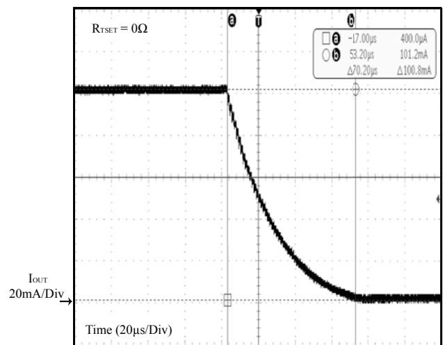
Figure 13 Instant Off
