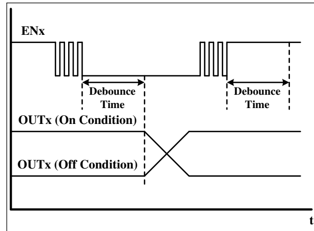
Figure 22 EN Debounced
