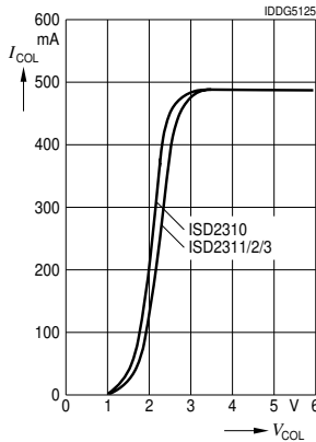
Peak Column Current vs. Column Voltage, ISD231X
