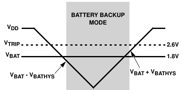
FIGURE 7. BATTERY SWITCHOVER WHEN V_{BAT} < V_{TRIP}
