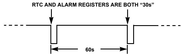
FIGURE 15. \overline{\text{IRQ}}/\text{FOUT} WAVEFORM
