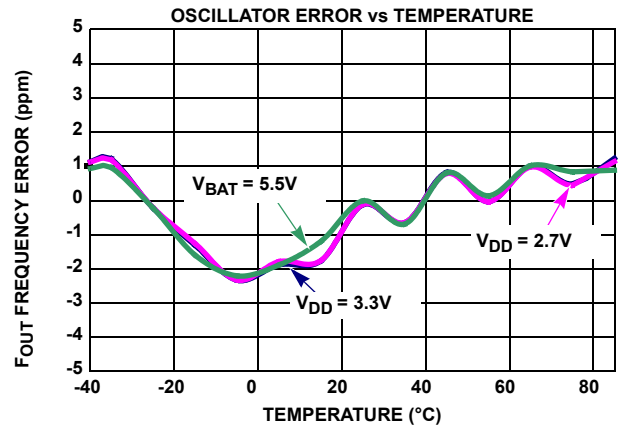
FIGURE 2. PERFORMANCE CURVE
