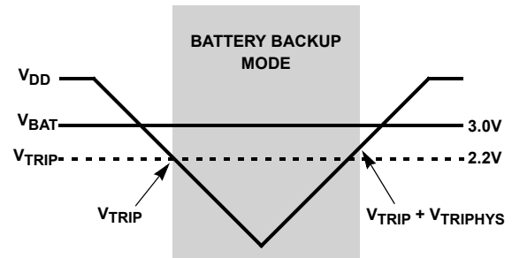
FIGURE 15. BATTERY SWITCHOVER WHEN V_{BAT} > V_{TRIP}
