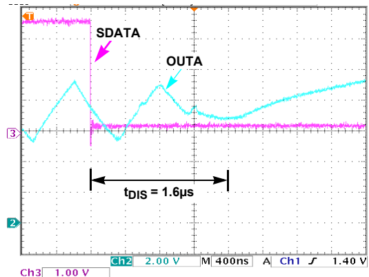
FIGURE 19. DISABLE RESPONSE
