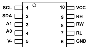
ISL22313 (10 LD MSOP) TOP VIEW
