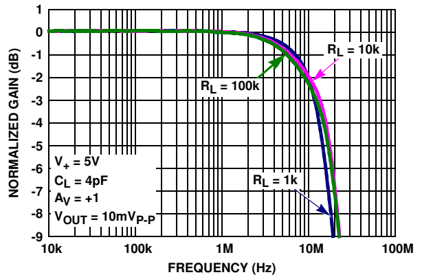
FIGURE 4. GAIN vs FREQUENCY vs R_L
