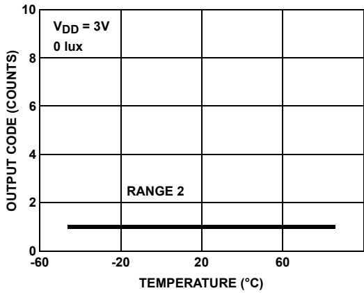
FIGURE 14. OUTPUT CODE FOR 0 LUX vs TEMPERATURE
