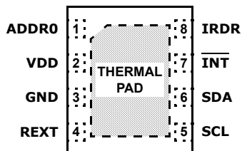
ISL29028 8 LD ODFN (2.0x2.1x0.7mm) TOP VIEW
