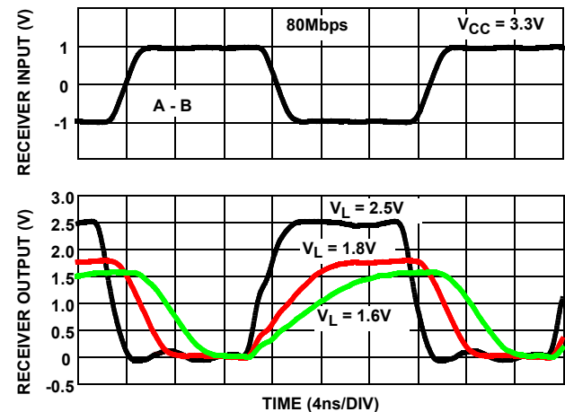
FIGURE 2. ISL3217XE DATA RATE AND V_L PERFORMANCE
