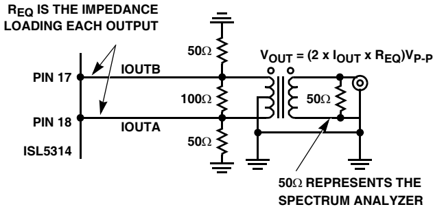
FIGURE 1. TRANSFORMER OUTPUT CIRCUIT OPTION
