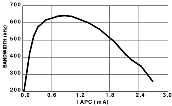
FIGURE 11. I OUT /I APC BANDWIDTH vs I APC
