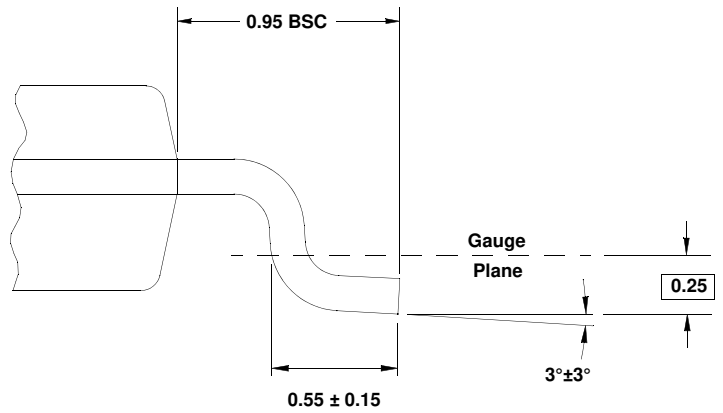
DETAIL "X"
