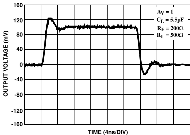
FIGURE 20. SMALL SIGNAL TRANSIENT RESPONSE
