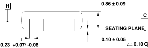
SIDE VIEW 1
