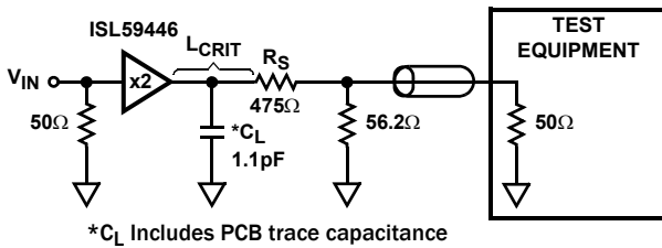
FIGURE 29C. 500Ω TEST CIRCUIT WITH 50Ω LOAD
