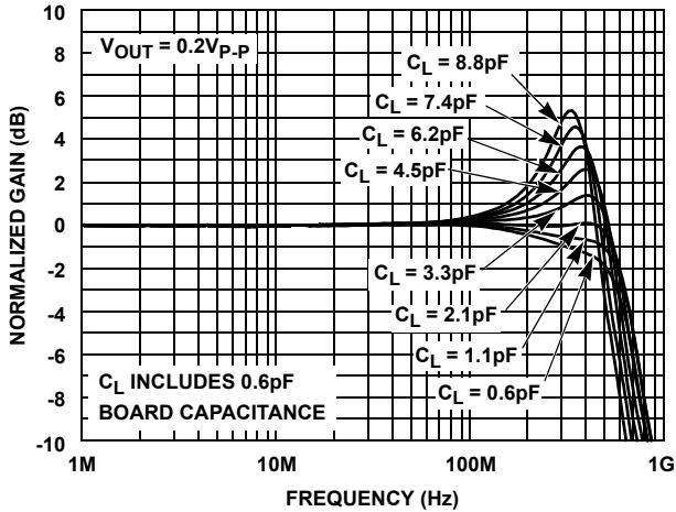
FIGURE 2. SMALL SIGNAL GAIN vs FREQUENCY vs C_L INTO 500\Omega LOAD
