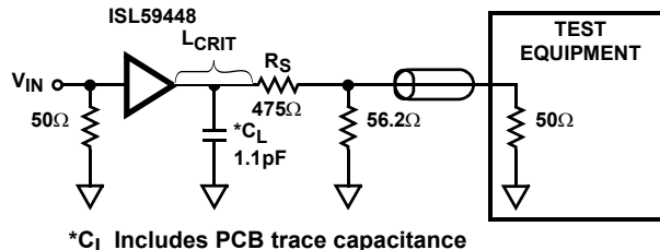
FIGURE 27C. 500Ω TEST CIRCUIT WITH 50Ω LOAD
