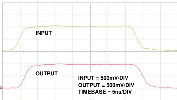
FIGURE 23. PULSE RESPONSE, GAIN = 1
