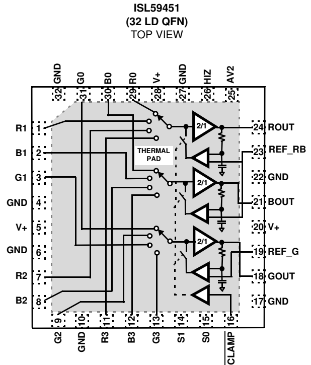
Exposed Thermal Pad (Gray Area) must be connected to GND.
