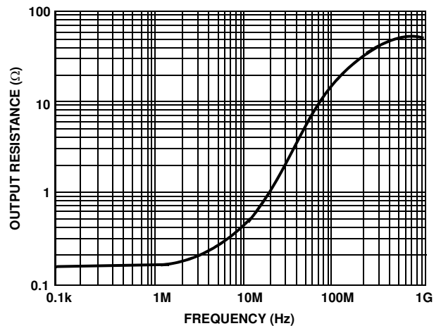
FIGURE 6. MUX1: R_{OUT} vs FREQUENCY
